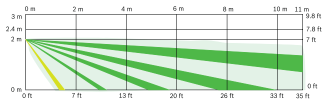
Fig. 2: Side view Broad 11 m x11 m (35 ft x 35 ft)
