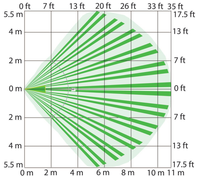
Fig. 1: Top View Broad 11 m x11 m (35 ft x 35 ft)
