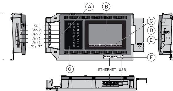
Fig. 1: Overview of panel controller
