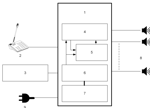
Schematic overview
