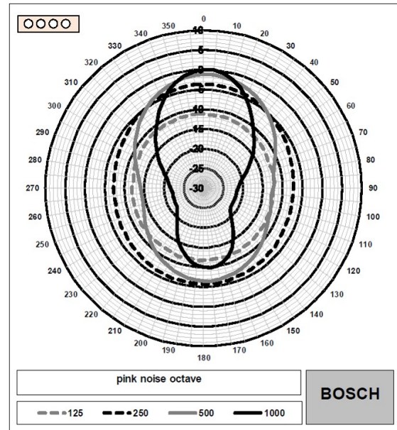
Fig. 6: Polar diagram LA2-UM60-L-IN (vertical measured with pink noise)
