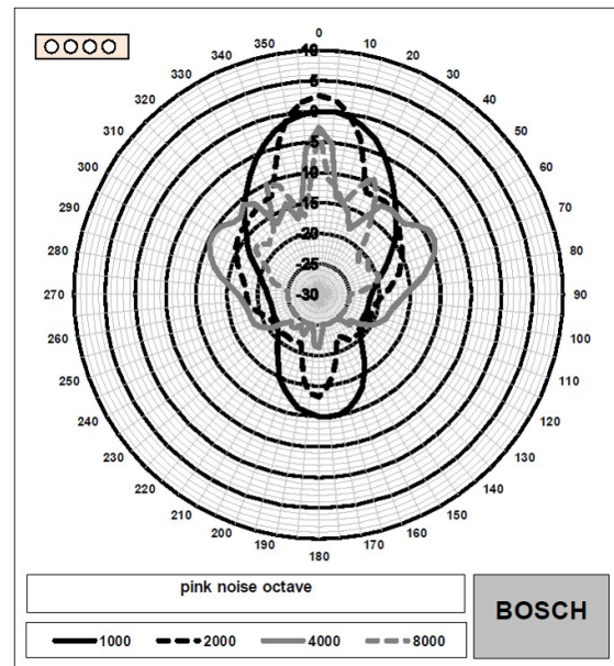
Fig. 7: Polar diagram LA2-UM60-L-IN (vertical measured with pink noise)
