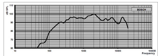
Fig. 3: Frequency response LA2-UM60-L-IN
