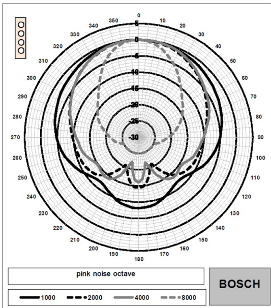
Fig. 5: Polar diagram LA2-UM60-L-IN (horizontal measured with pink noise)
