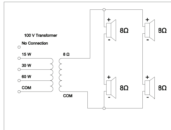
Fig. 2: Circuit diagram LA2-UM60-L-IN
