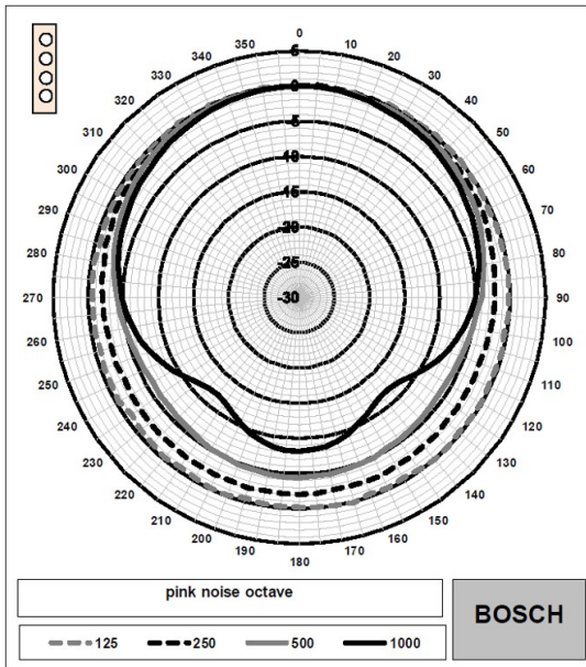
Fig. 4: Polar diagram LA2-UM60-L-IN (horizontal measured with pink noise)
