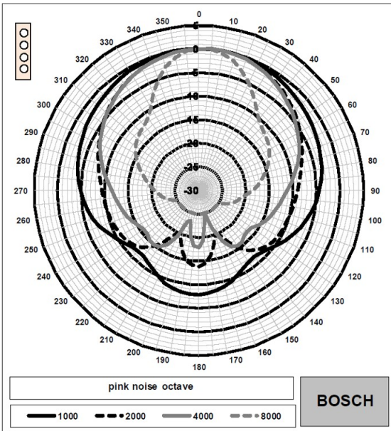
Fig. 5: Polar diagram LA2-UM40-LZL-IN (horizontal measured with pink noise)
