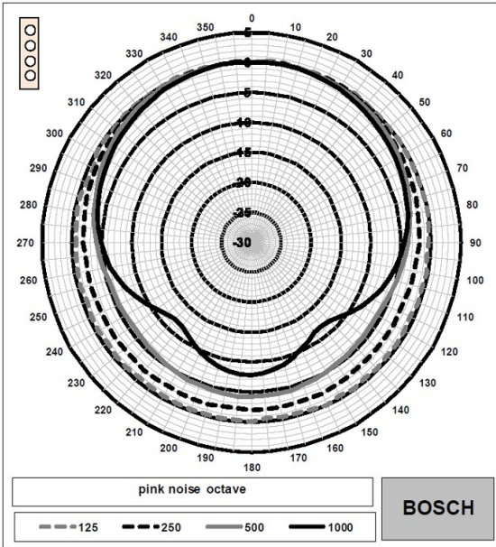
Fig. 4: Polar diagram LA2-UM40-LZL-IN (horizontal measured with pink noise)
