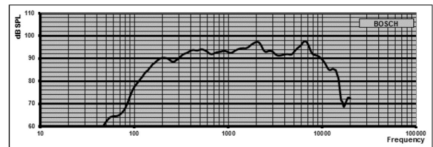
Fig. 3: Frequency response LA2-UM40-LZL-IN
