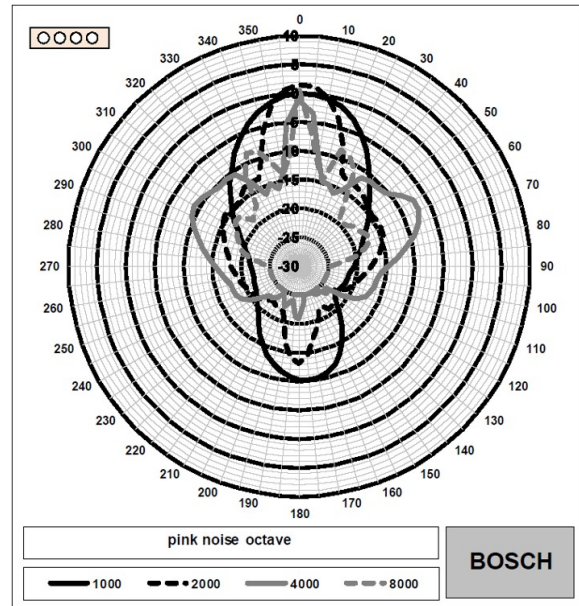
Fig. 7: Polar diagram LA2-UM40-LZL-IN (vertical measured with pink noise)
