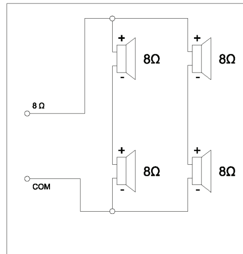
Fig. 2: Circuit diagram LA2-UM40-LZL-IN
