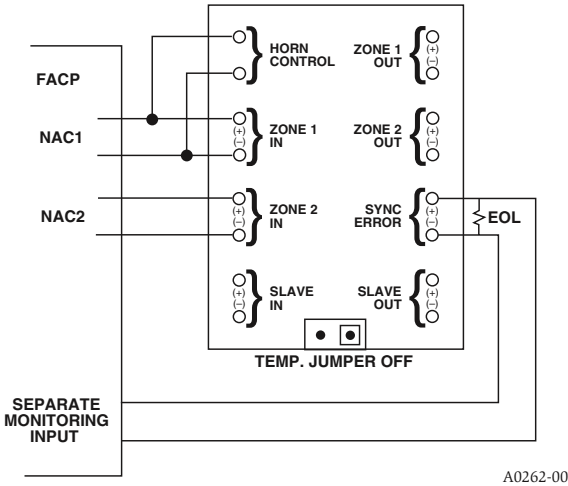
Figure 4: Multiple Devices Using Sync Error
