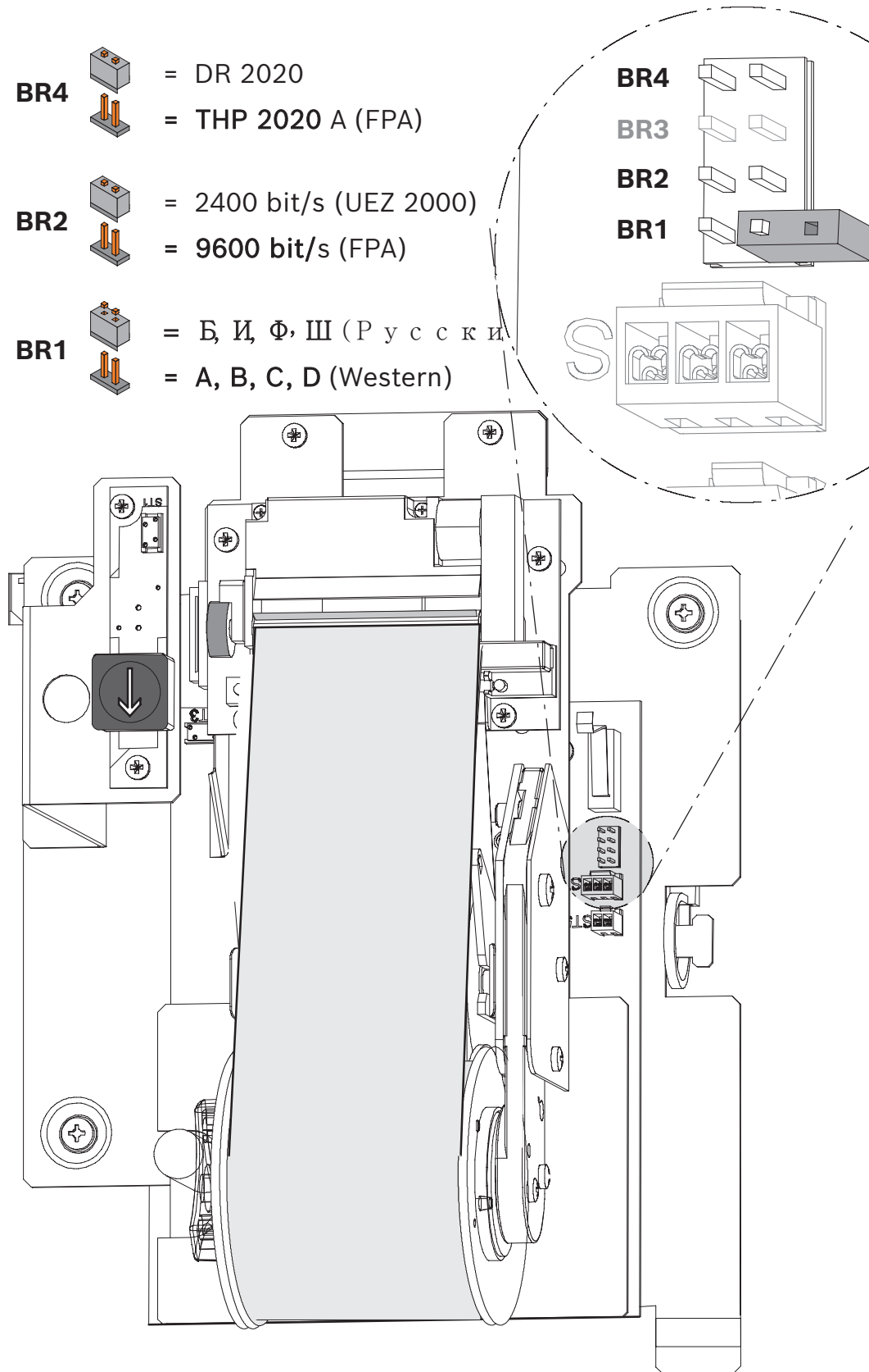
Figure 4.77: THP 2020 A jumpers
