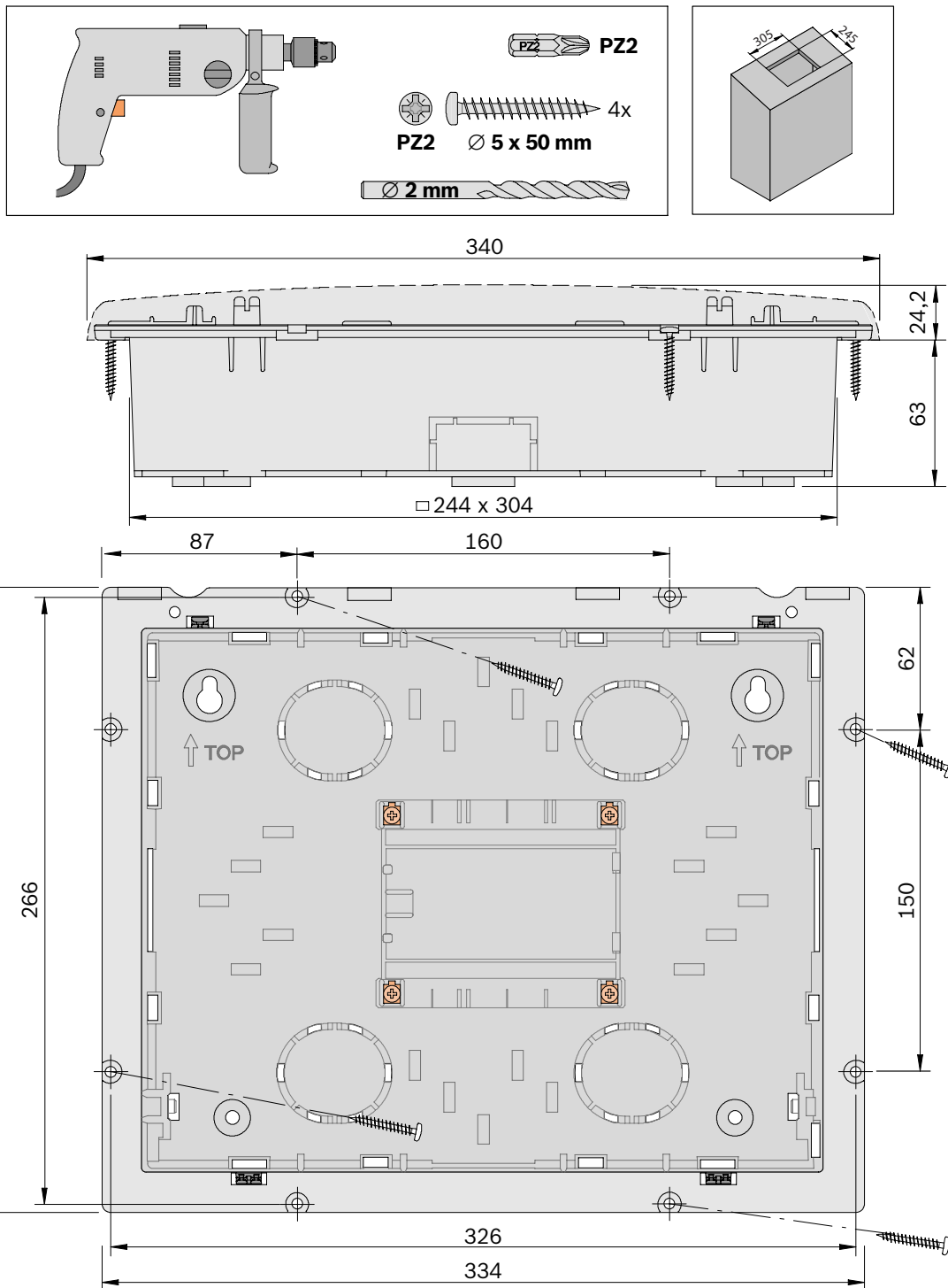
Figure 4.87: Remote Keypad tilting installation; dimensions in mm
