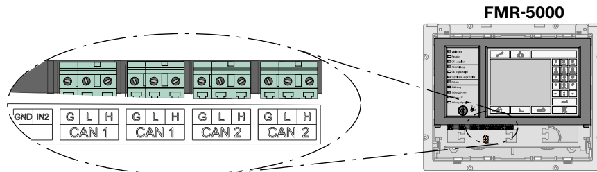
Figure 4.92: Network Connections
