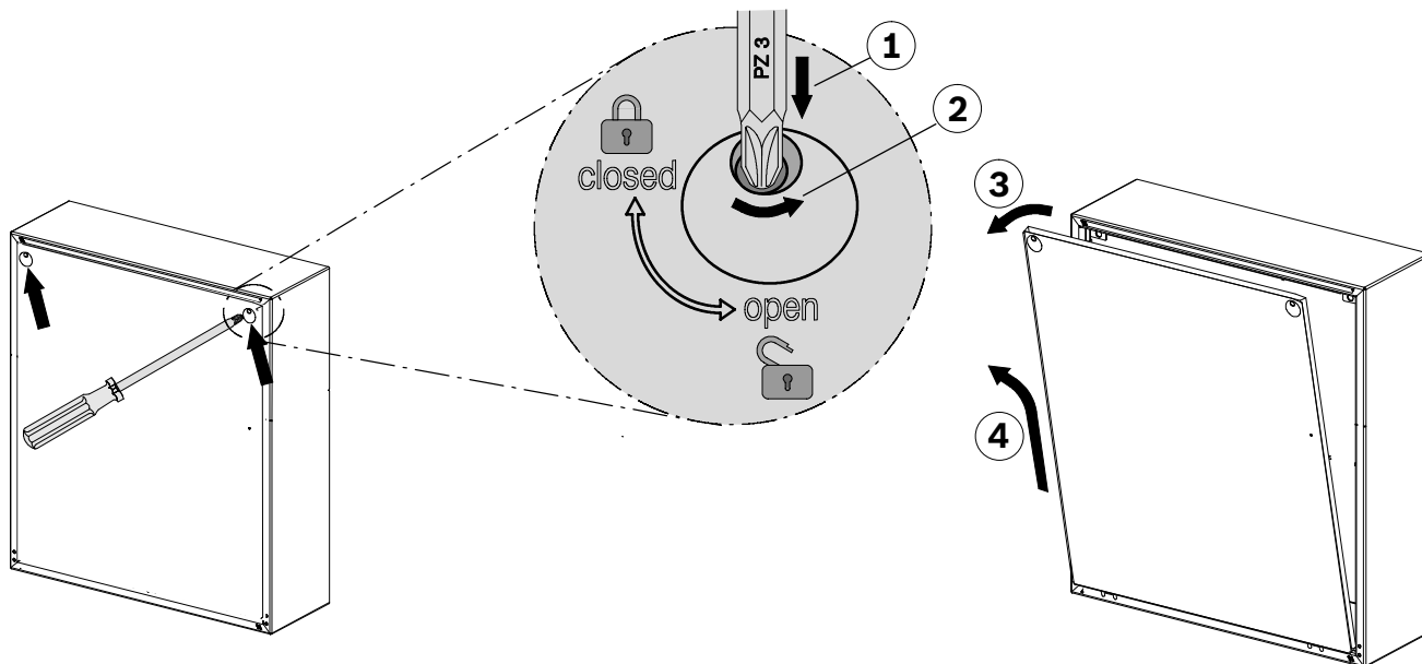
Figure 4.21: FPO-5000-PSB-CH/FPO-5000-PSB1 installation (1-4)
