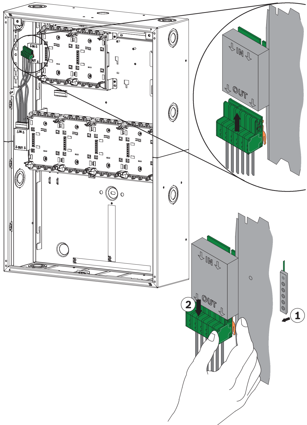
Figure 4.36: Connection of panel rail
