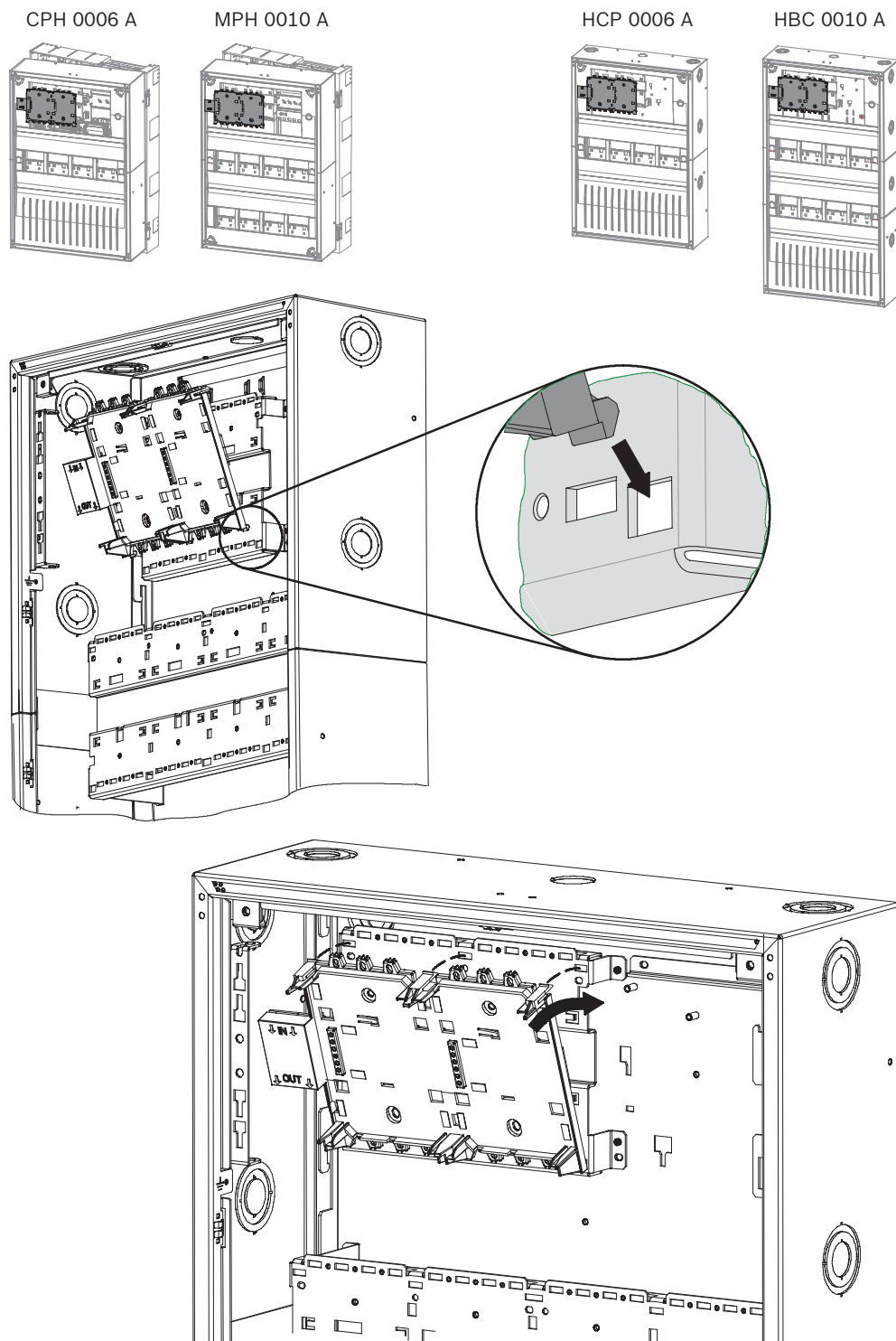
Figure 4.35: PRS-002-C installation
