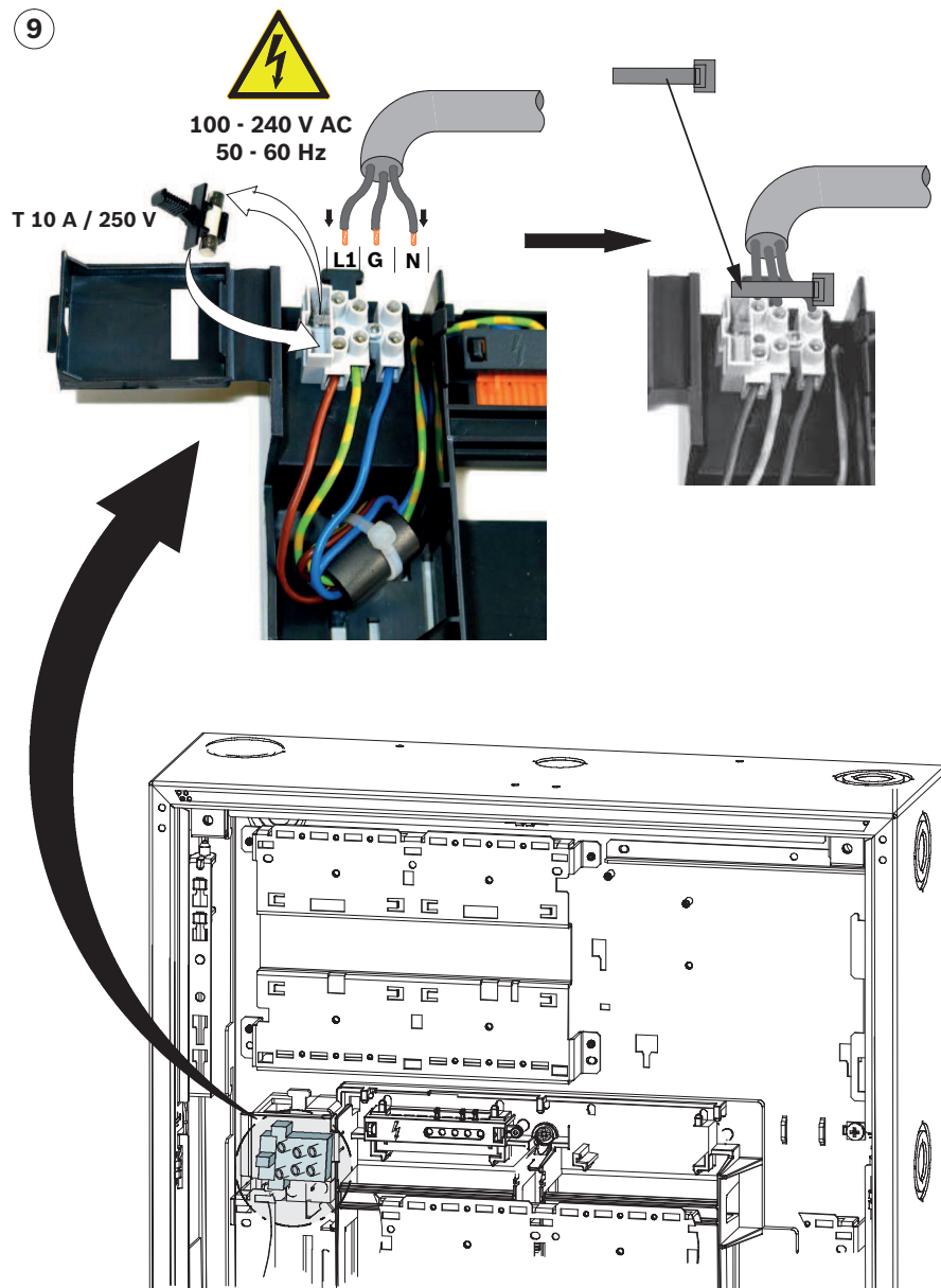
Figure 4.25: FPO-5000-PSB-CH installation (9)
