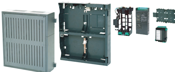
Figure 4.73: FPP-5000 External Power Supply Unit Kit 24 V/6 A
