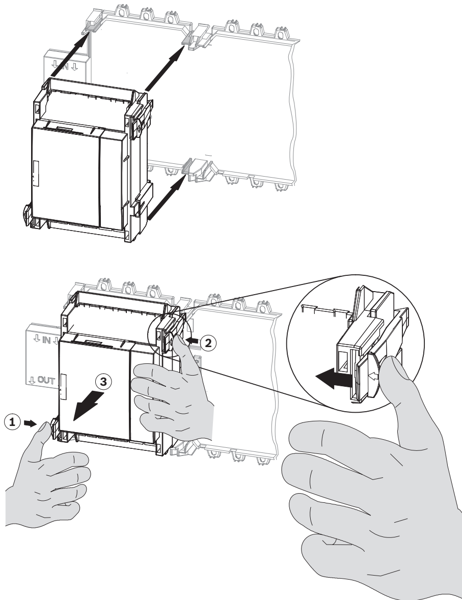
Figure 4.49: Installation and removal of functional modules
