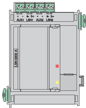
Figure 4.63: LSN 0300 A LSN improved Module 300 mA
