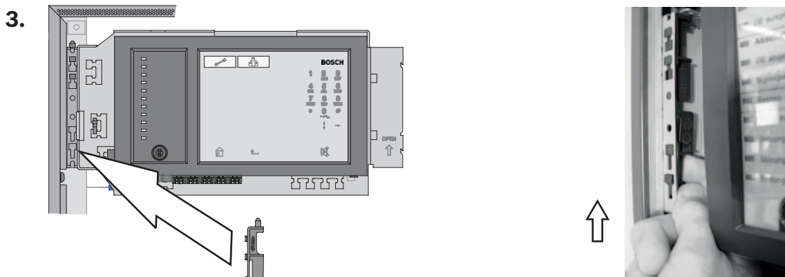
Figure 4.43: MPC installation (1-3)
