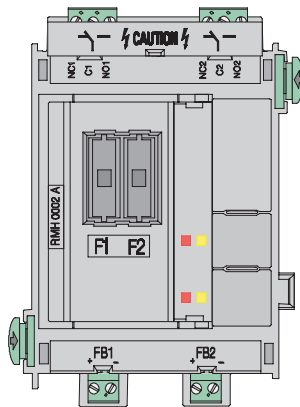
Figure 4.67: RMH 0002 A Relay Module for mains voltage
