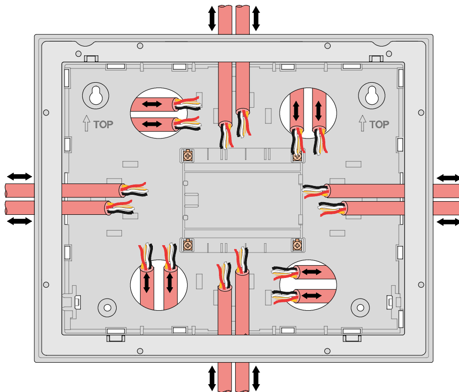
Figure 4.84: Remote Keypad installation (11-13)
