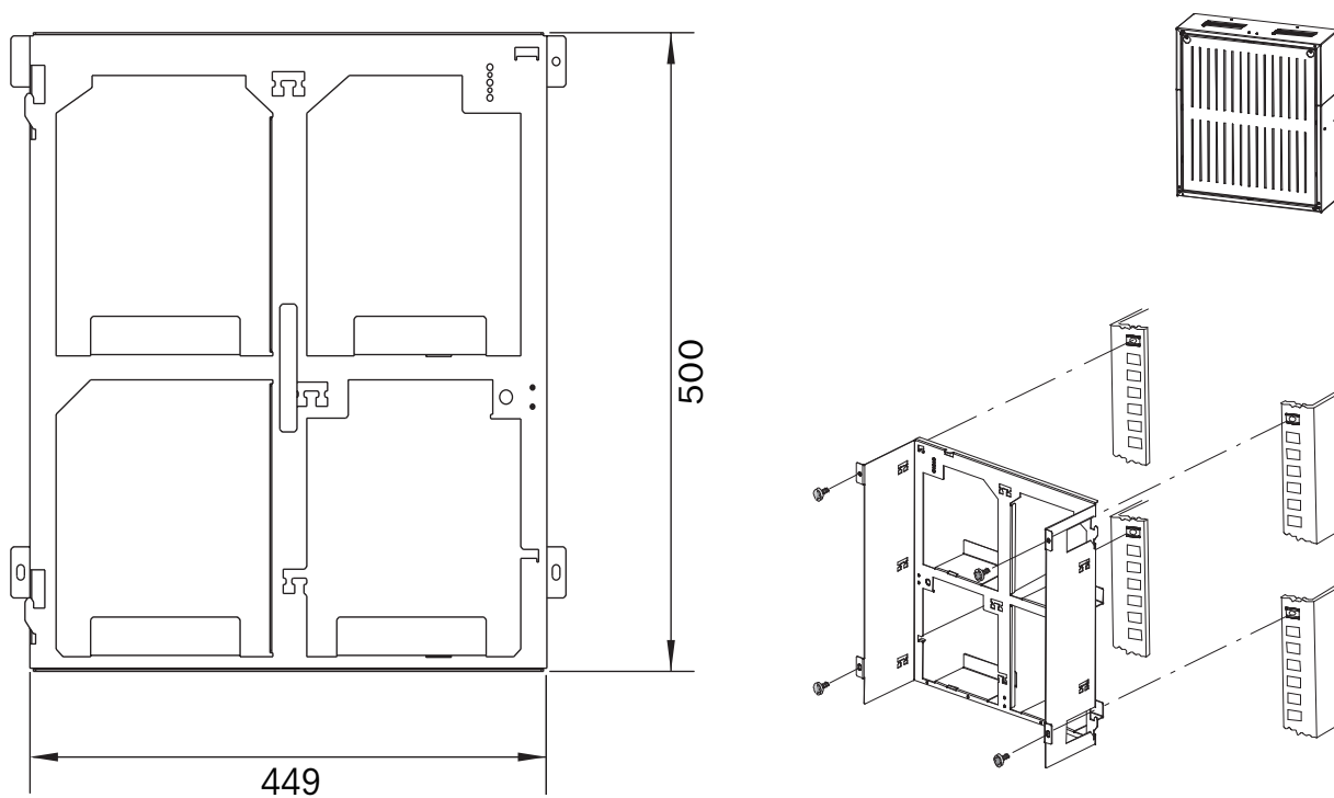
Figure 4.15: FRM 0019 A installation kit for PMF 0004 A [installation dimensions in mm]
