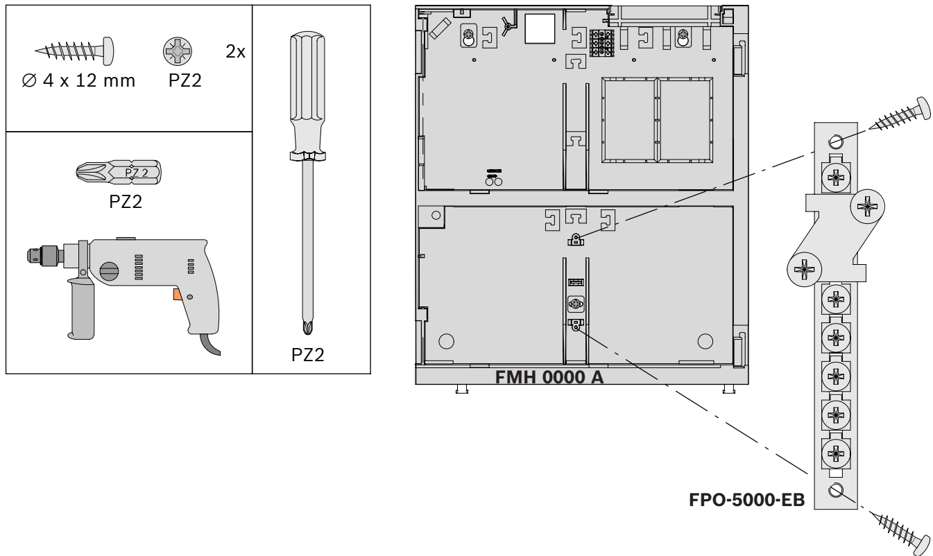
Figure 4.20: FPO-5000-EB installation
