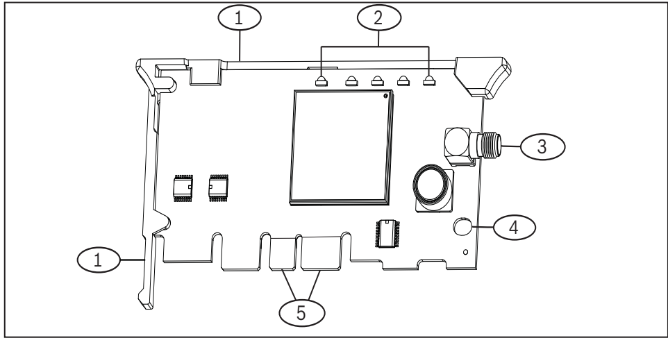
Figure 1.1: Module overview
