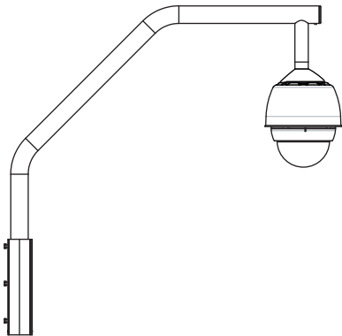
图 8.6: VGA-ROOF-MOUNT
